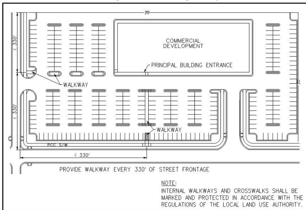
Figure 3.5.4.3-a Locating Walkways
