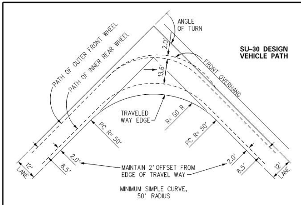
Figure 5.2.5.1-c Simple Curve Radius Example for a SU-30
