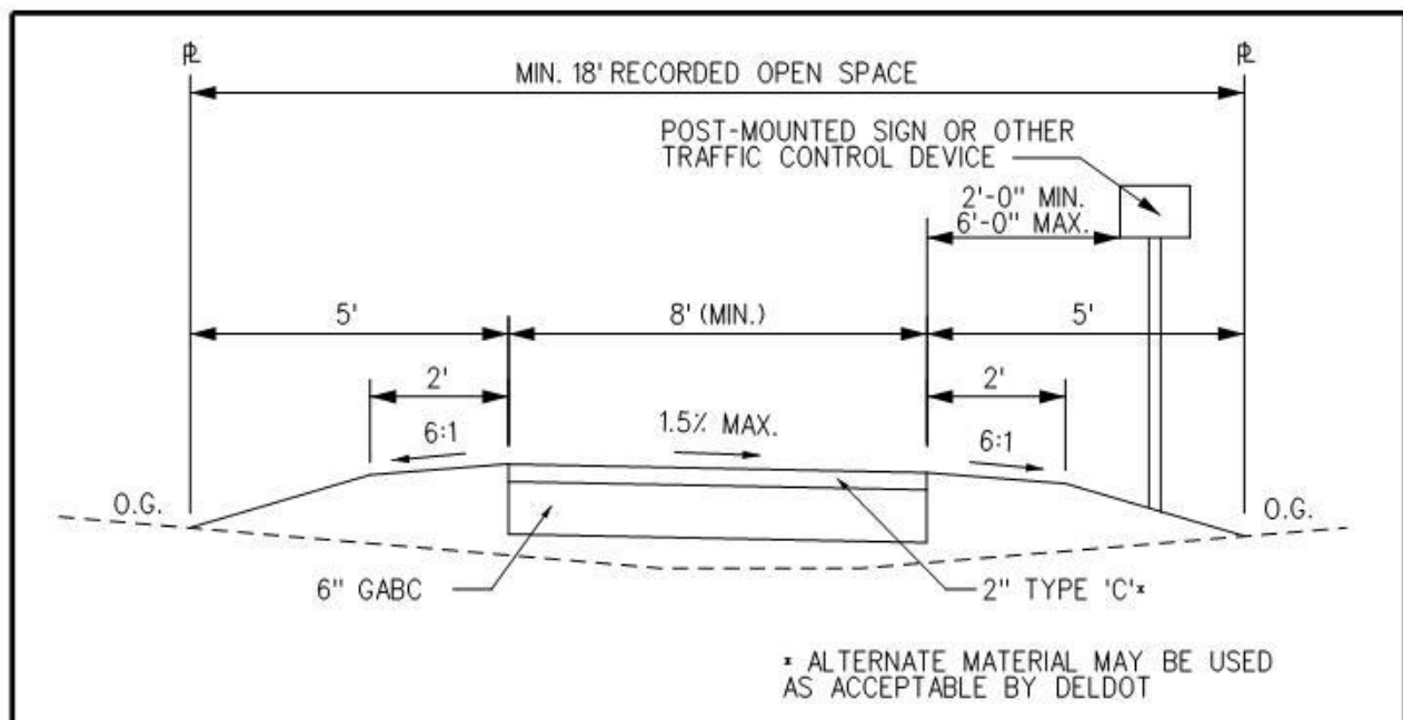
Figure 3.5.4.4-a Access-way Width
