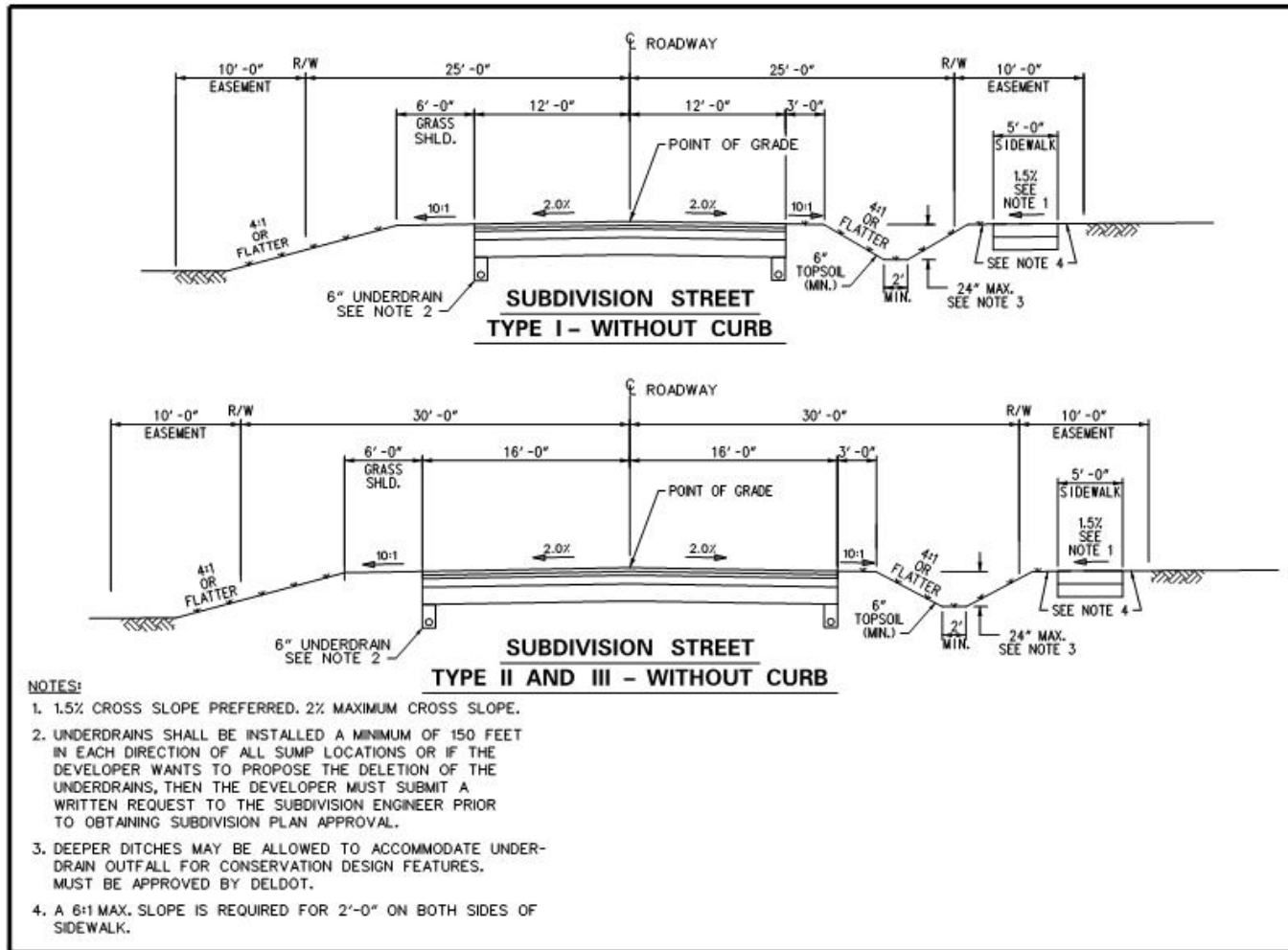
Figure 5.5.2-c Subdivision Street Typical Section (Without Curb) (Not to Scale)
