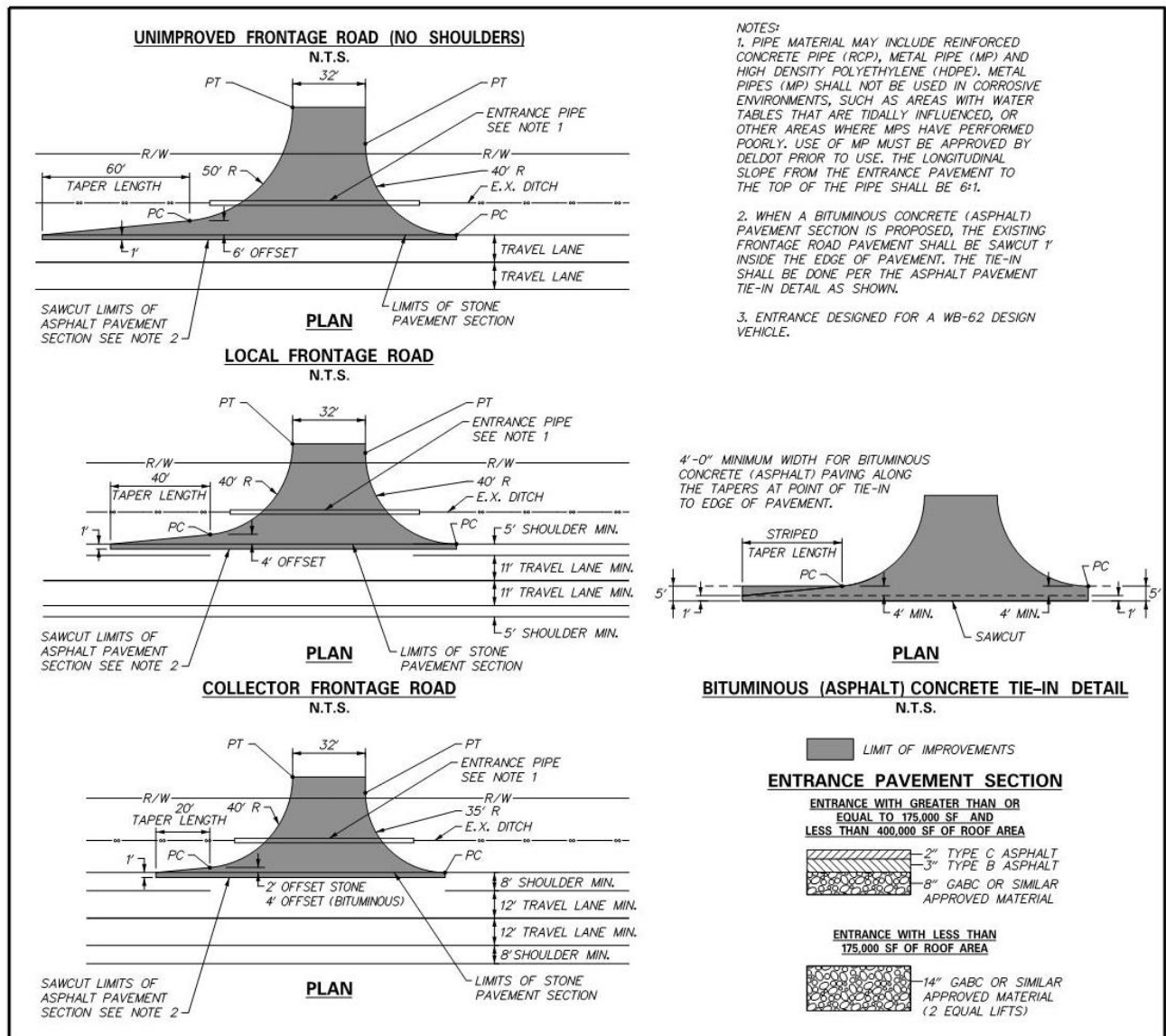
Figure 8.5.2-a Agricultural Entrance Detail
