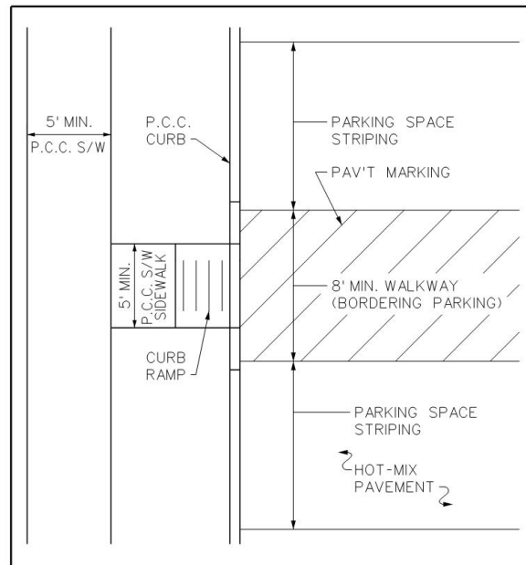
Figure 3.5.4.3-b Walkway Routing
