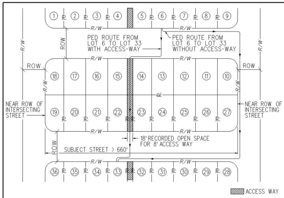
Figure 3.5.4.4-b Access-ways – 660' < Block Length < 1320'
