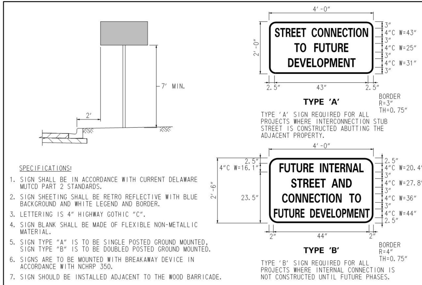
Figure 5.1.5.2-b Stub Street Sign Detail
