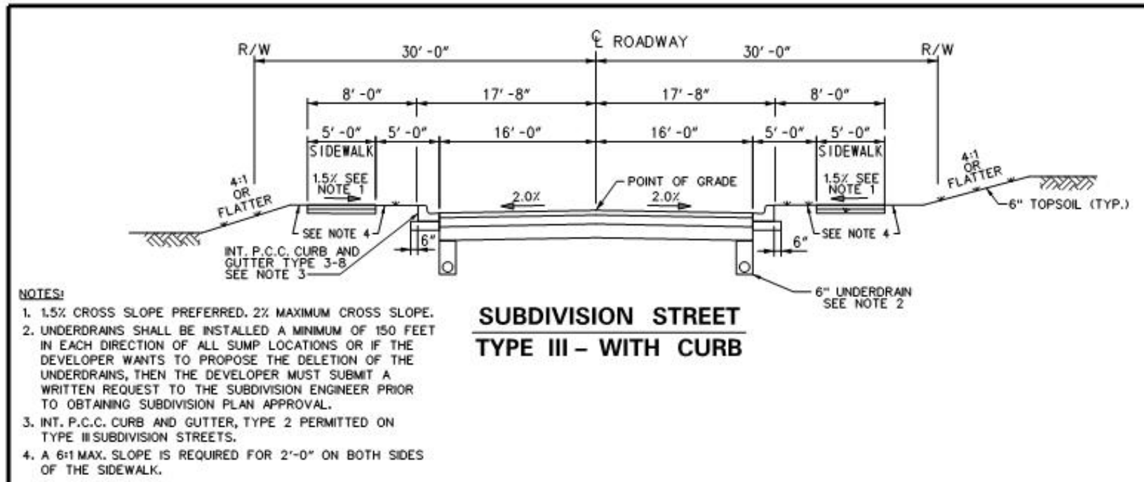
Figure 5.5.2-b Subdivision Street Typical Section (With Curb) - Type III (Not to Scale)
