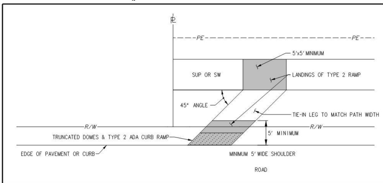
Figure 3.5.4.2-b Sidewalk/Shared Use Path Tie-in
