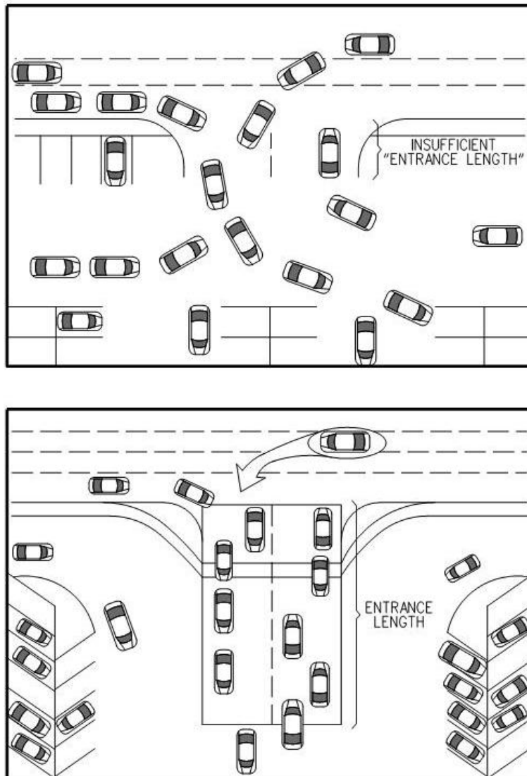
Figure 5.2.6-a Entrance Length Example
